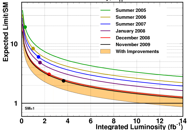
CDF Run II Preliminary, m_H=115 GeV
