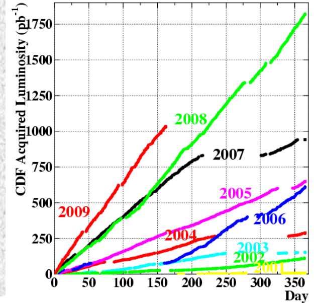
Collider Run II Integrated Luminosity
