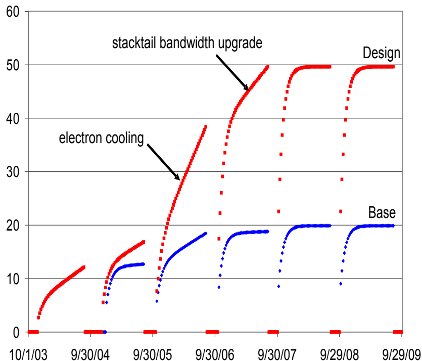
Integrated Weekly Luminosity (pb-1)
