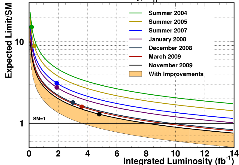
CDF Run II Preliminary, m_H=160 GeV
